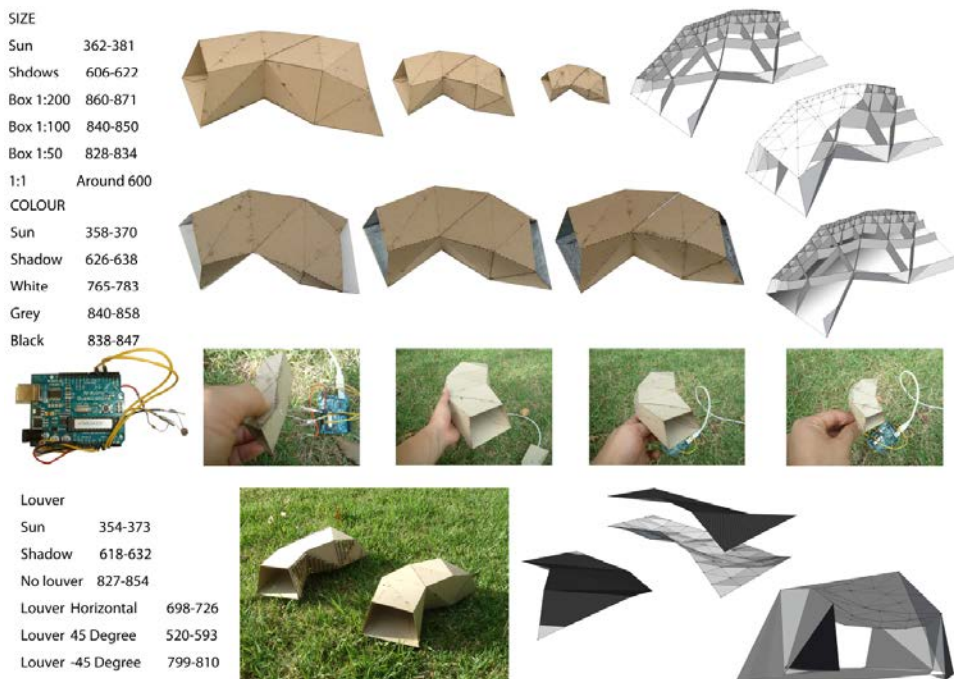
FIG 19: Ambient light analysis using Arduino and light sensors being placed inside the physical models.
