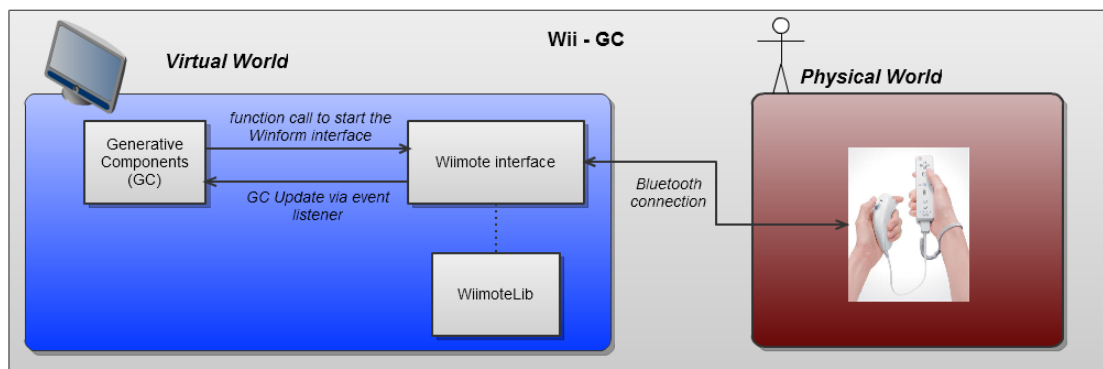
FIG 5: The software architecture of the Wiimote-GC experiment
