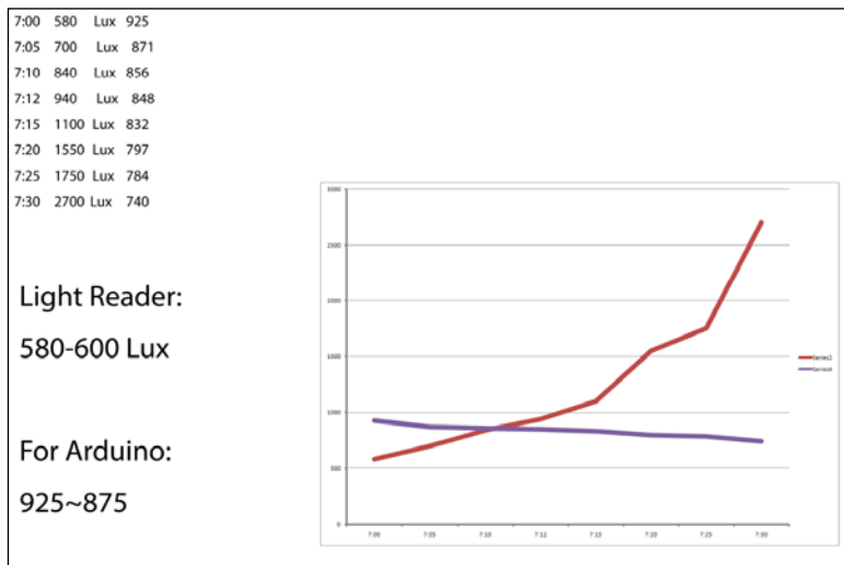
FIG 18: The calibration of the light sensor data and light reader.
